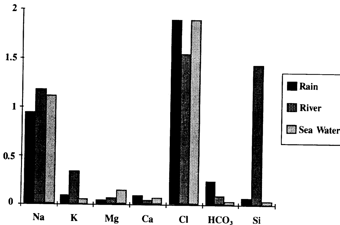
Figure 1. The Composition of Rio Tefé Water (mg/1), Rainwater in the Rio Tefé Basin (mg/1) and Sea Water ((g/1)/(10)) (from Gibbs, 1970).
