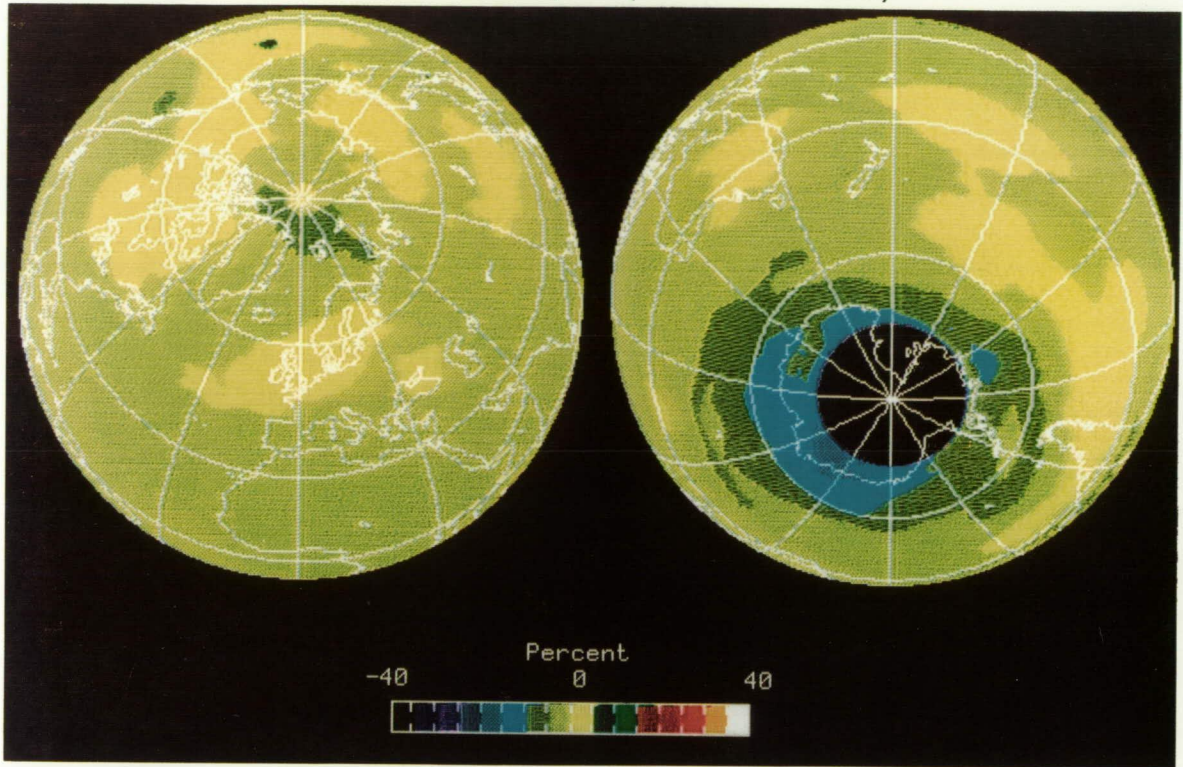
TOTAL OZONE CHANGE FOR SEPTEMBER (1987 + 1986) — (1980 + 1979)
