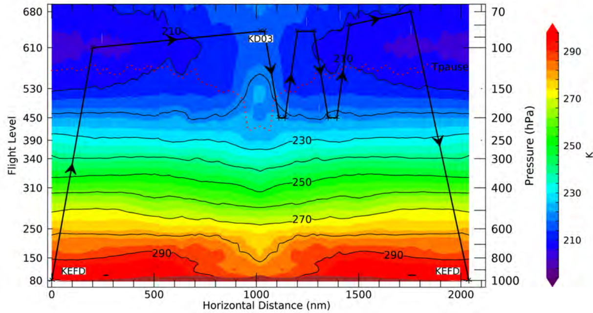
NCEP Temperature Init:2026080406 Valid Time:2026080406
