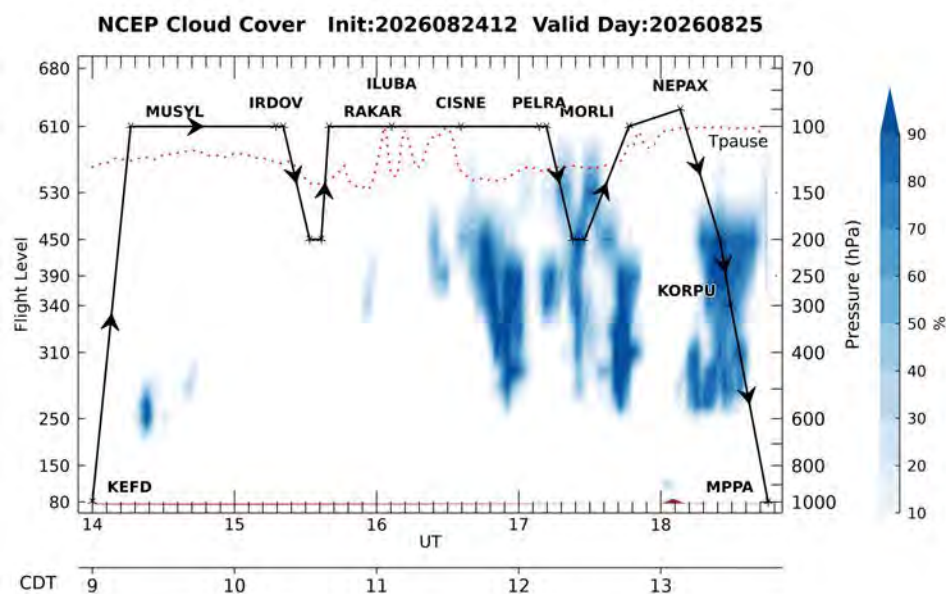
Cloud Cover
